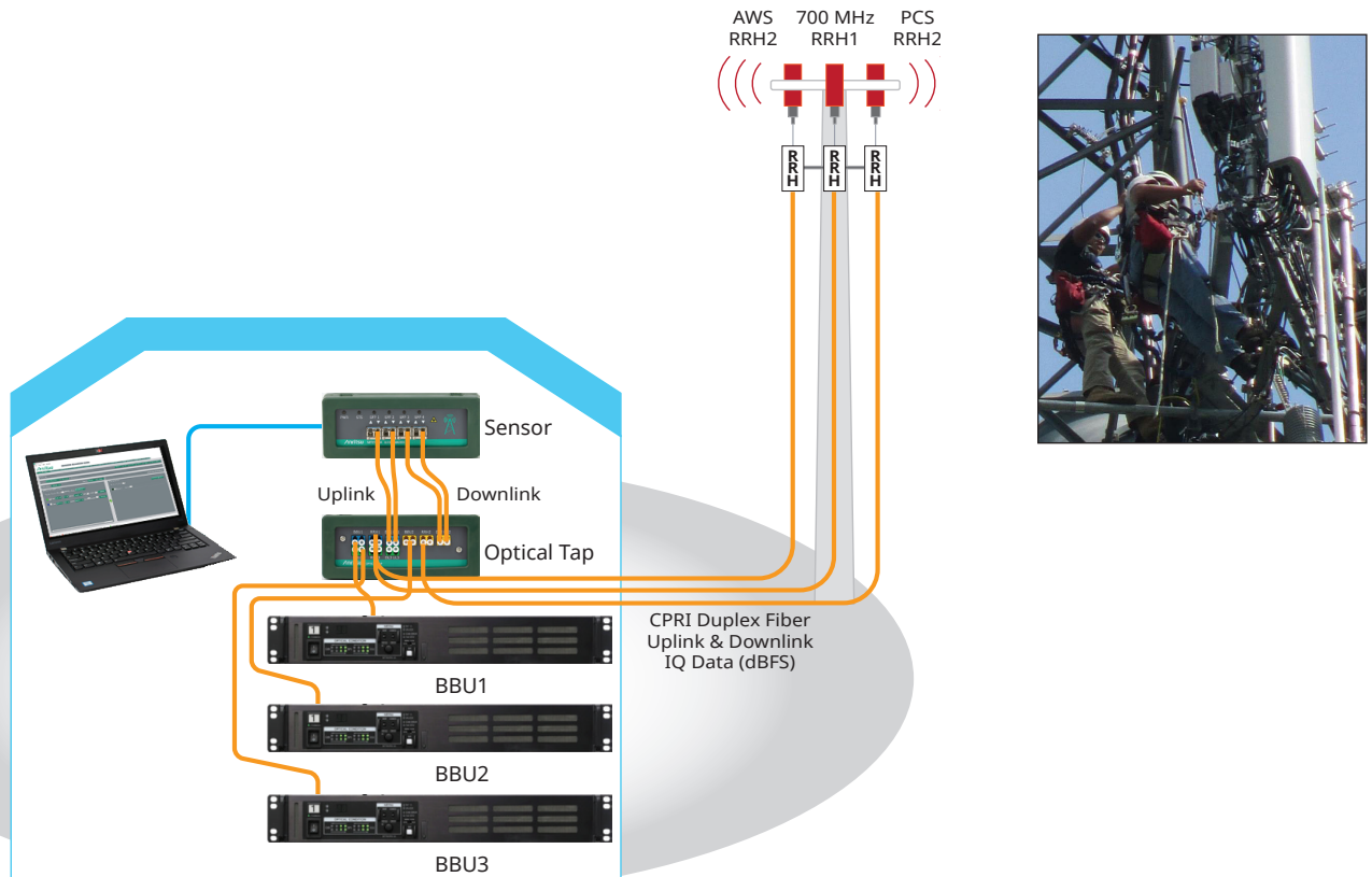
Multi-Band Connection Diagram
